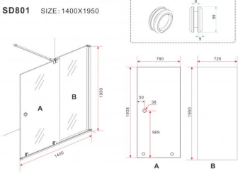
SD801 SIZE: 1400X1950
