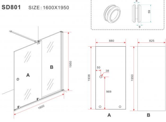
SD801 SIZE: 1600X1950
