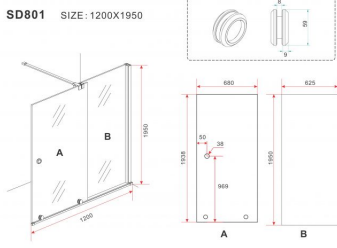
SD801 SIZE: 1200X1950
